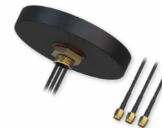
Combo SISO mobile/GNSS/Wi-Fi roof SMA antenna Order code: PR1KCS28
