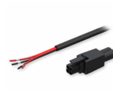
Power cable with 4-way open wire Order code: PR2PL15B
